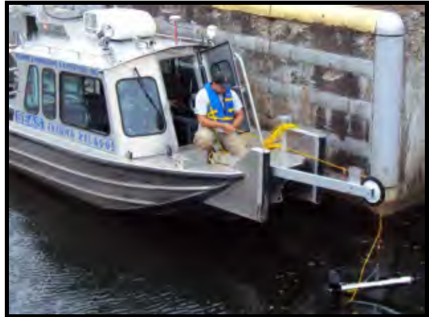
EdgeTech Towfish mounted off the bow
