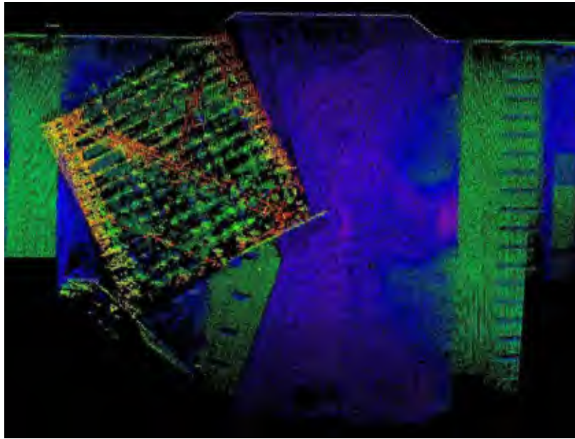
Figure N-11. Multibeam survey of Markland Lock Gate that broke free and fell into the lock sill. Detailed surveys allowed the district to determine the damage to the gate and if it could be safely removed without dewatering the chamber. (Louisville District)
