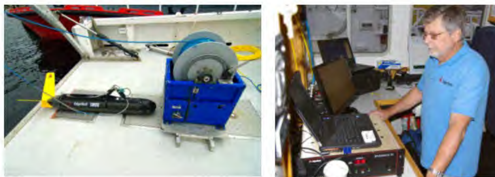
Figure Q-2. Basic components of a side scan sonar system. (left) Towfish and tow cable on winch. (Right) Sonar interface box and computer. (EdgeTech)
