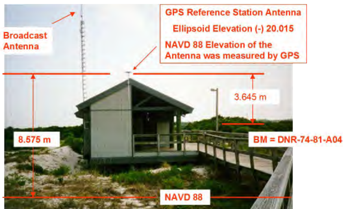
Figure H-4. RTK reference base station parameters.
