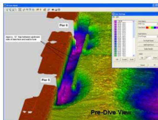
Figure N-3. On left, initial plan of multibeam survey at Mel Price Lock & Dam (Mississippi River). Significant scour (15 to 20 ft below normal grade) was indicated at piers 5, 6, 9, and 10). On right, 3D detail model of Pier 5 and 6 scour area furnished to divers. (St. Louis District)
