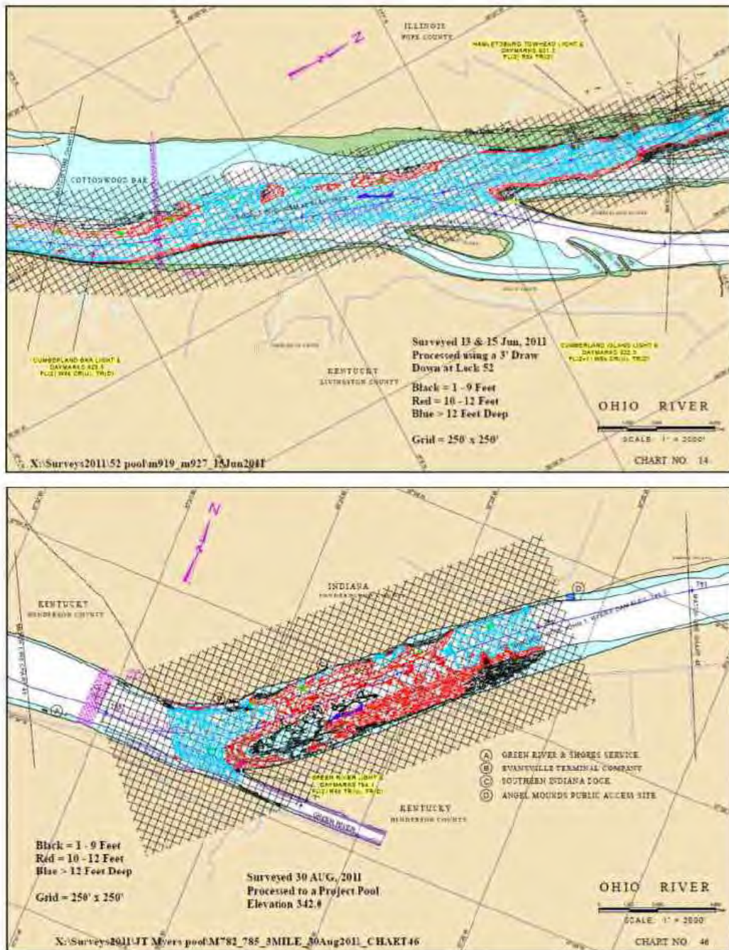
Figure N-13. Louisville District surveys of pools on the Ohio River. Depths below 12 feet are color-coded in red and black.
