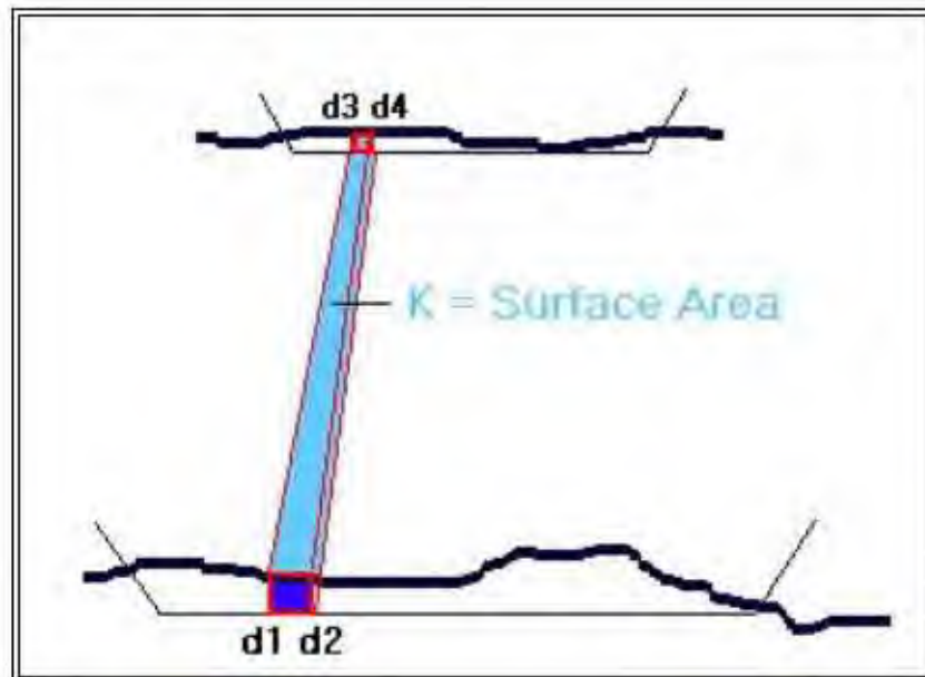
Figure 10-16. Standard HYPACK prismoidal end area and volume computation method.
