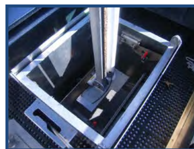
Multibeam in Moon Well
