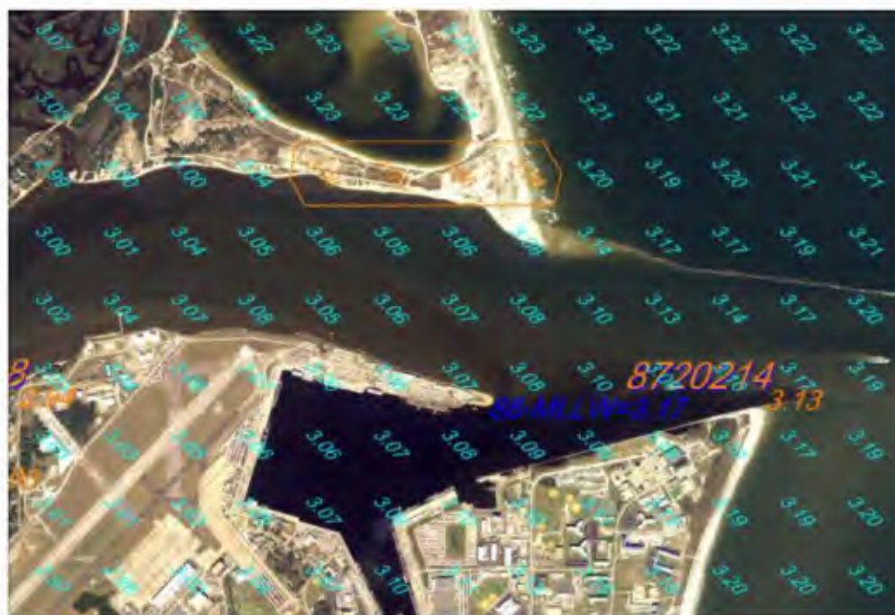
Figure 7-6. Example of a KTD file generated from VDatum. (Ocean entrance to Mayport Naval Base, St. Johns River, FL). “K” values are “NAVD88 – MLLW.” Note incorrect VDatum and KTD interpolation on north side of entrance, between the river and tidal pool. This region required manual edits to the KTD file to correct. Published NOAA gage 8720214 “K” at South Jetty agrees closely with VDatum “K.”
