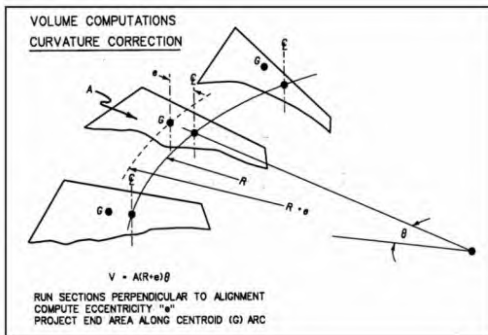
Figure 10-23. Curved channel volume computations.
