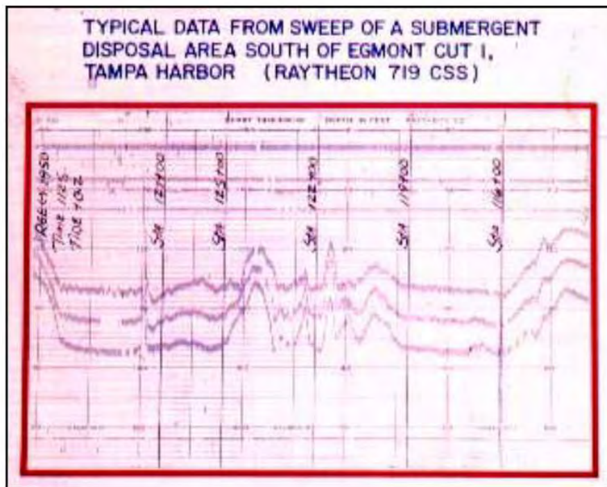
Figure 5-11. Raytheon 719 CSS multiple transducer analog record ca 1980. (Jacksonville District)
