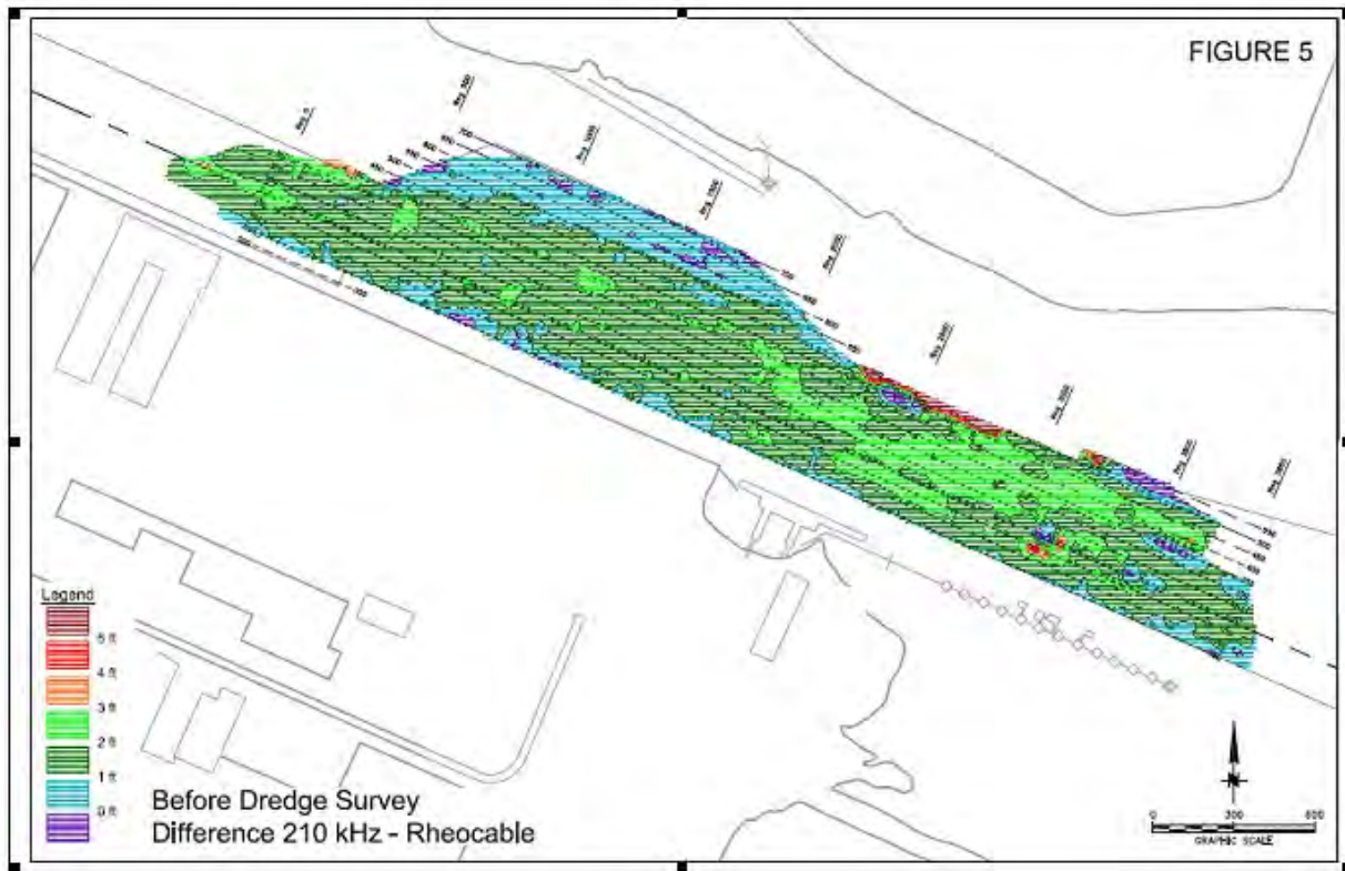
Figure P-18. Difference plot between Rheocable and 33-kHz depth measurements demonstrated in Wilmington Harbor, DE.
