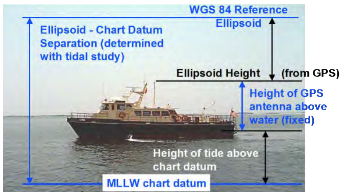
Figure H-5. RTK measurements on survey vessel
