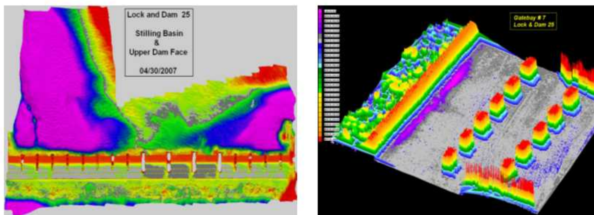
Figure N-5. Multibeam survey of Lock and Dam 25 (Mississippi River). Expanded 3D details showing a scour area and baffle blocks below gate 7. (St. Louis District)
