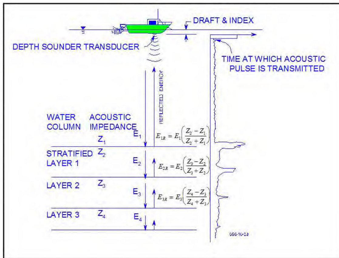
Figure P-4. Acoustic impedance (Z) and acoustic reflectivity (E) changes in differing sediment densities.
