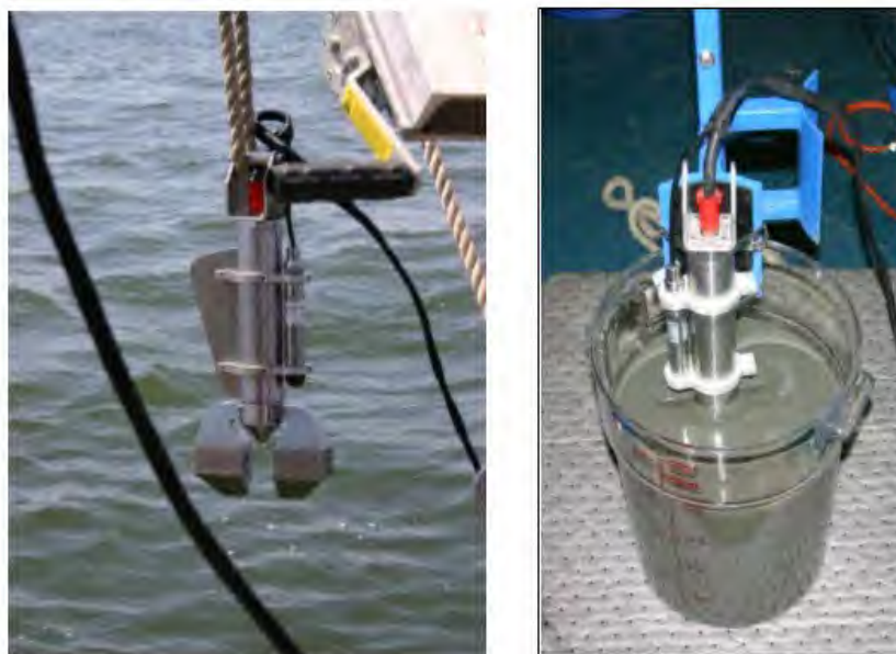
Figure P-13 High Resolution Density Profiler (HRDP) and its immersion in a static (fluid mud) bucket test.
