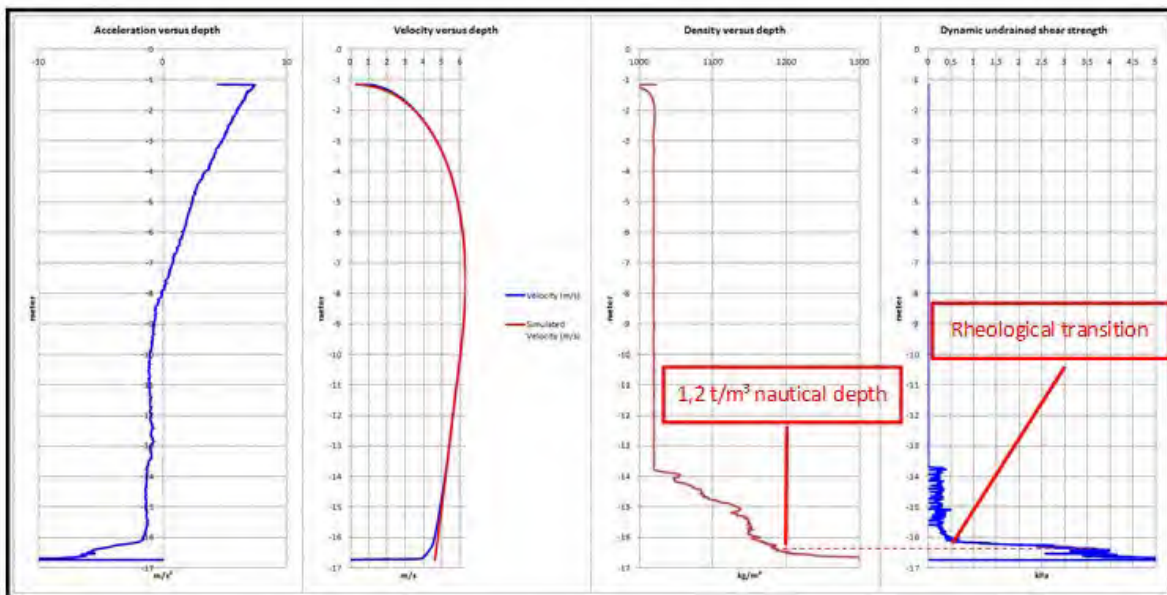
Figure P-15 GraviProbe profile of density and shear strength vs. depth.
