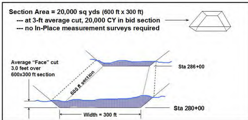
Figure 10-2. Station Dredging.
