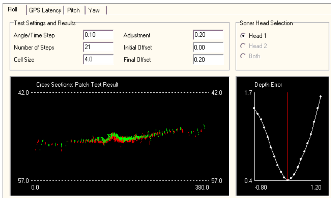
Figure F-1. Preliminary Patch Test: Roll Bias = 0.15 degrees:
